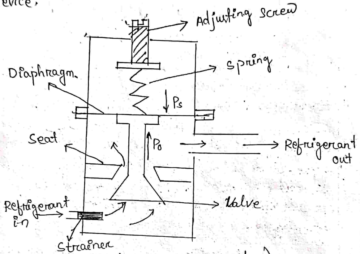
(Automatic expansion valve)
