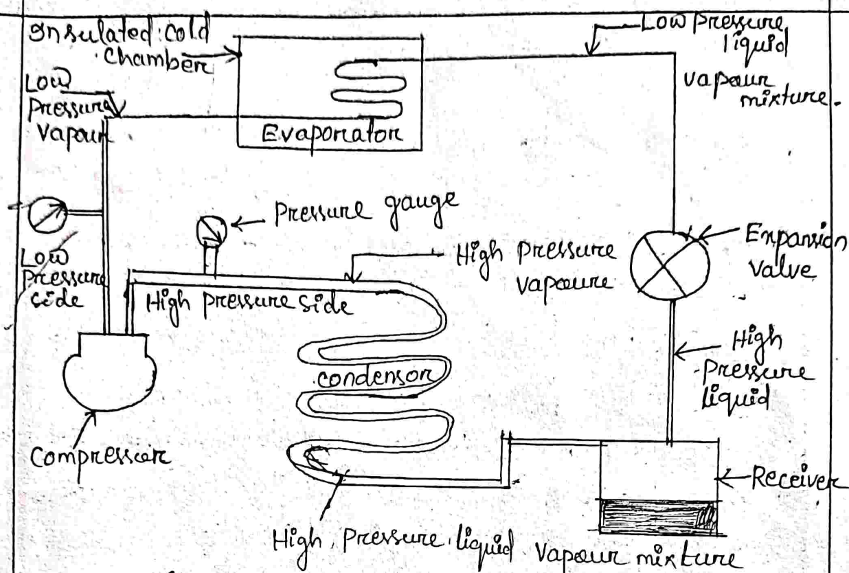
(Vapour compression refrigerator)
