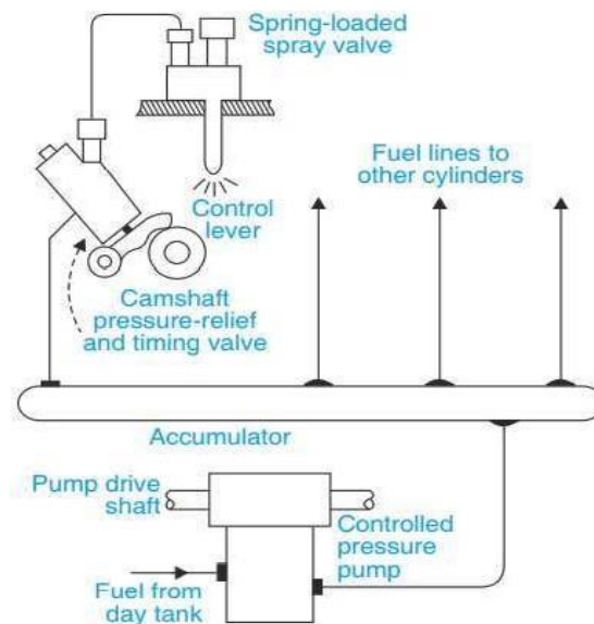
Figure: Common Rail Fuel Injection System
